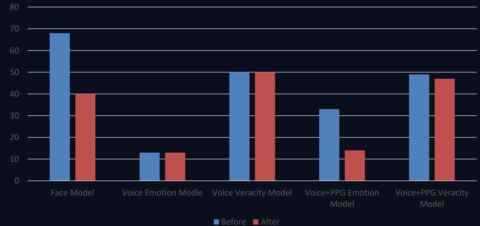
Accuracy
