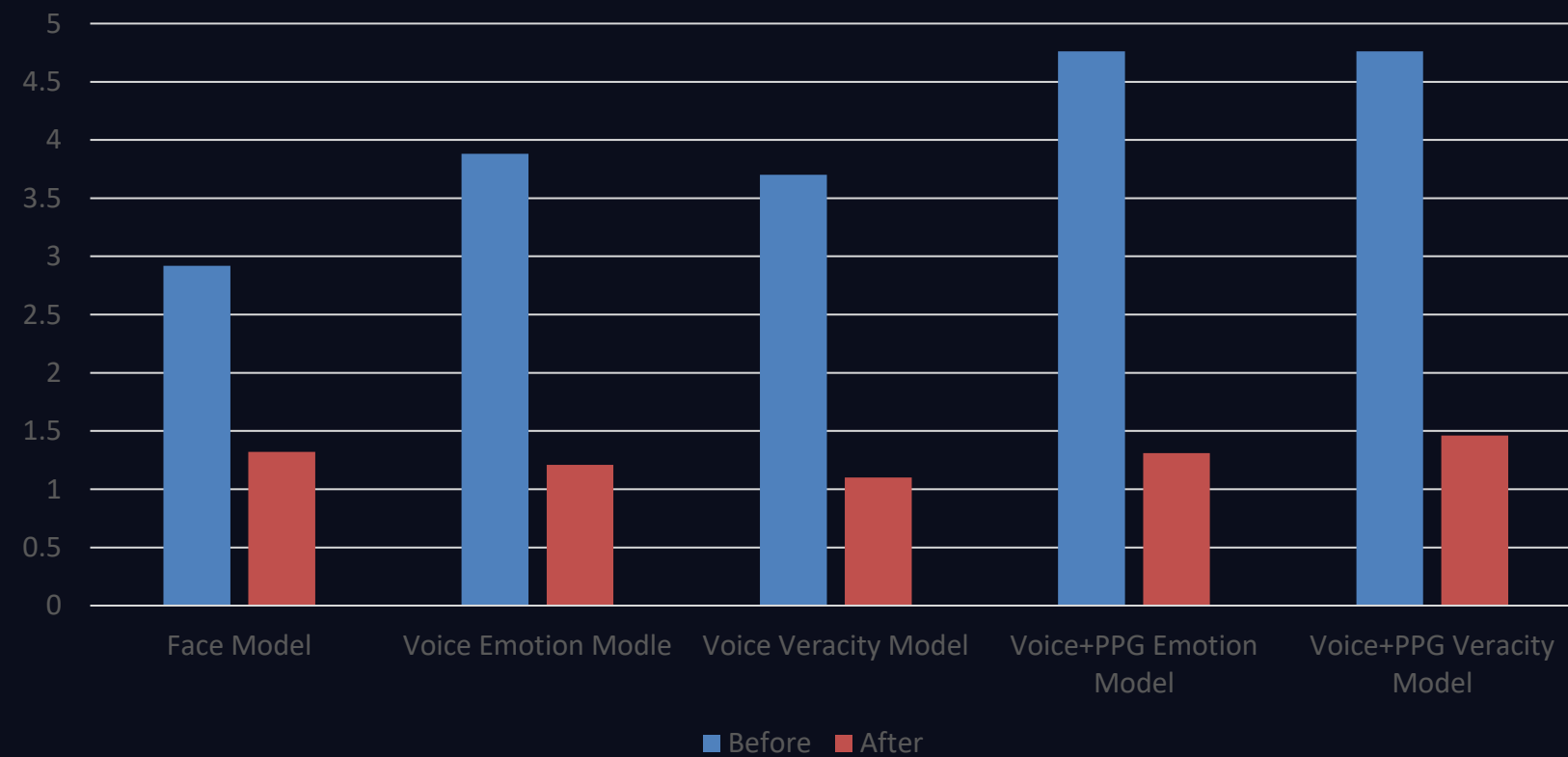
Model size
